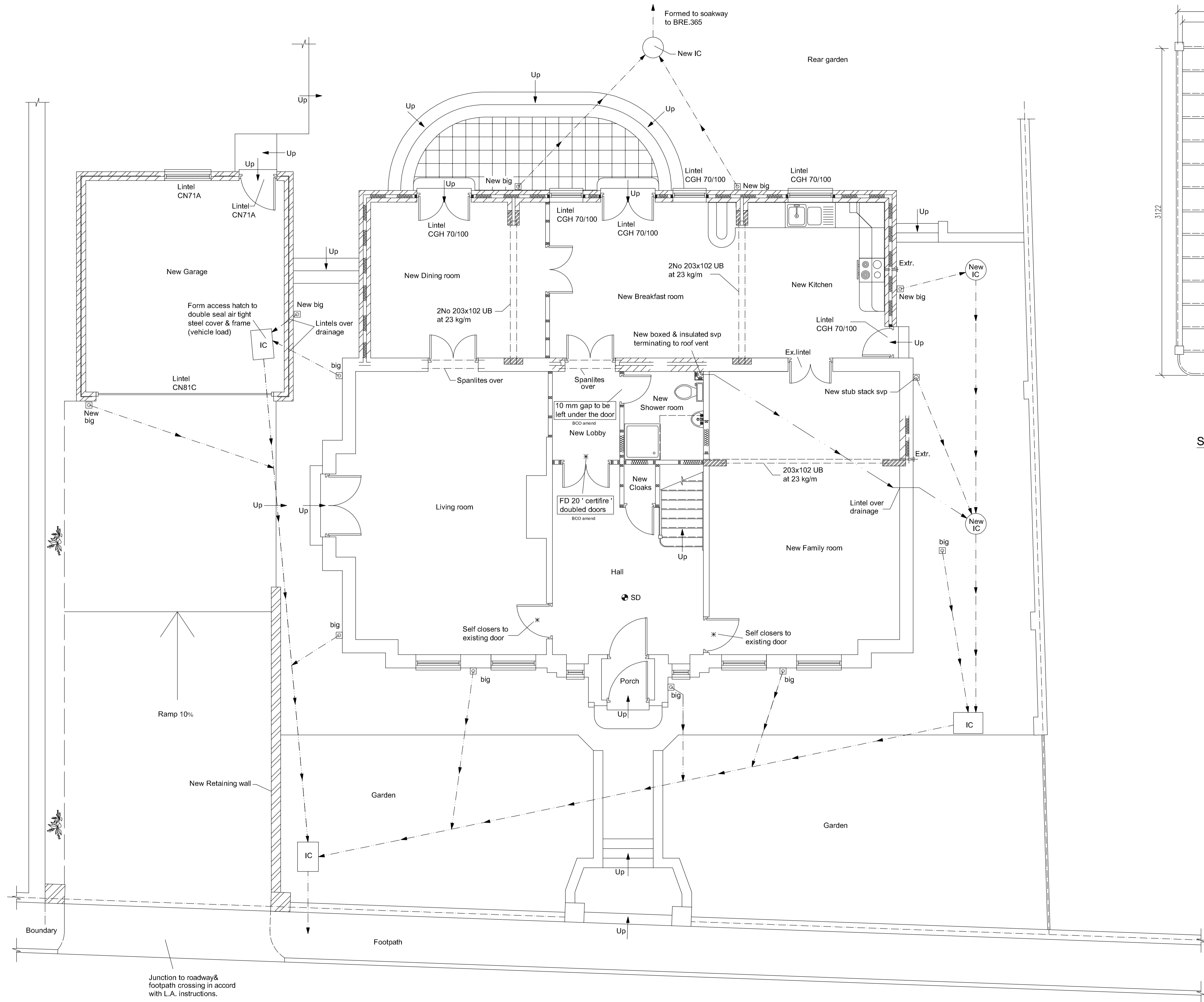
PROPOSED GROUND FLOOR PLAN
