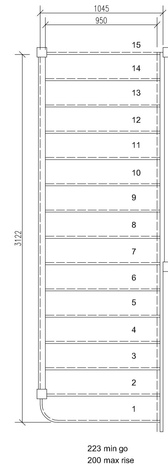
STAIR DETAIL
